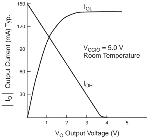
Figure 13. Output Drive Characteristics of MAX 9000 Devices Notes (1), (2)
