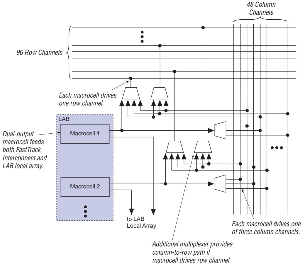
Figure 7. MAX 9000 LAB Connections to Row & Column Interconnect
