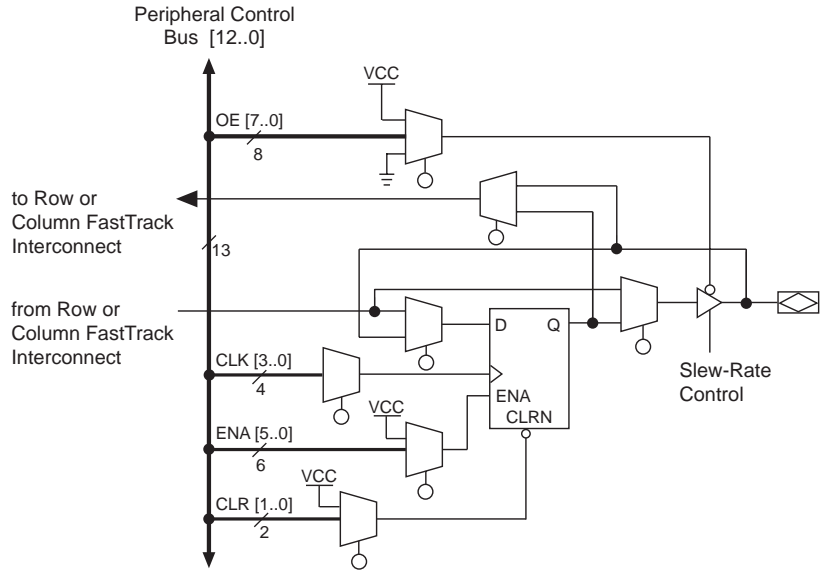
Figure 10. MAX 9000 IOC
